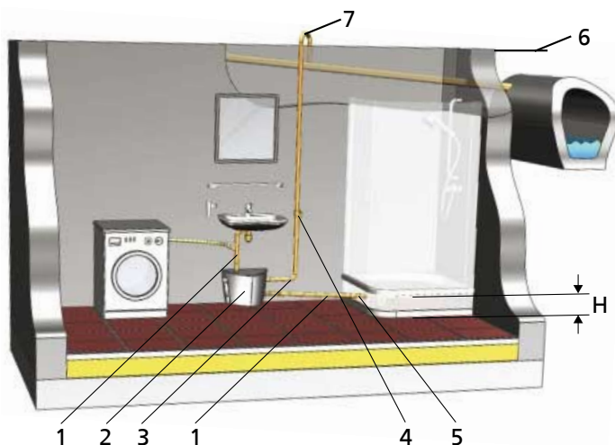
Fig. 3: Installation example
