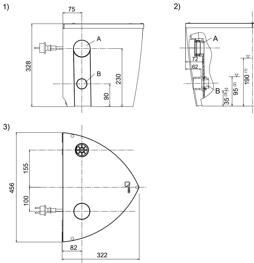
Fig. 1: Dimensions [mm]
